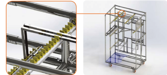
Item name : Case top chassis Parts : STS Pipe, AL2820, Rubber guide(FSB-2) Load Q'ty : 23EA
