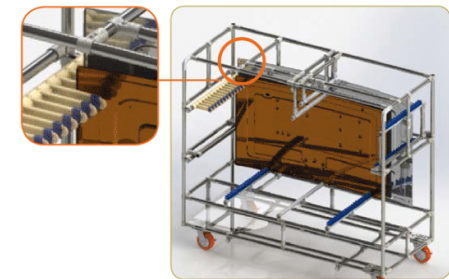
Item name : Cover bottom Parts : STS-Pipe, Rubber guide(G-type), DJP-400/400S Load Q'ty : 20EA
